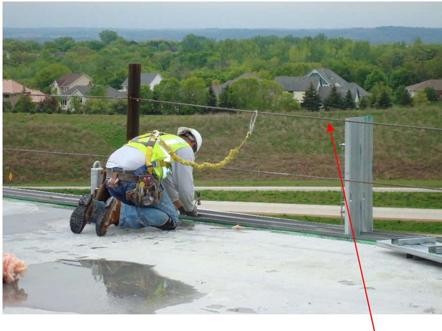
Perimeter guardrail system with engineered fall protection for top rail, missing flagging every six feet
